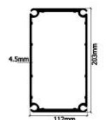
Main frame profile
